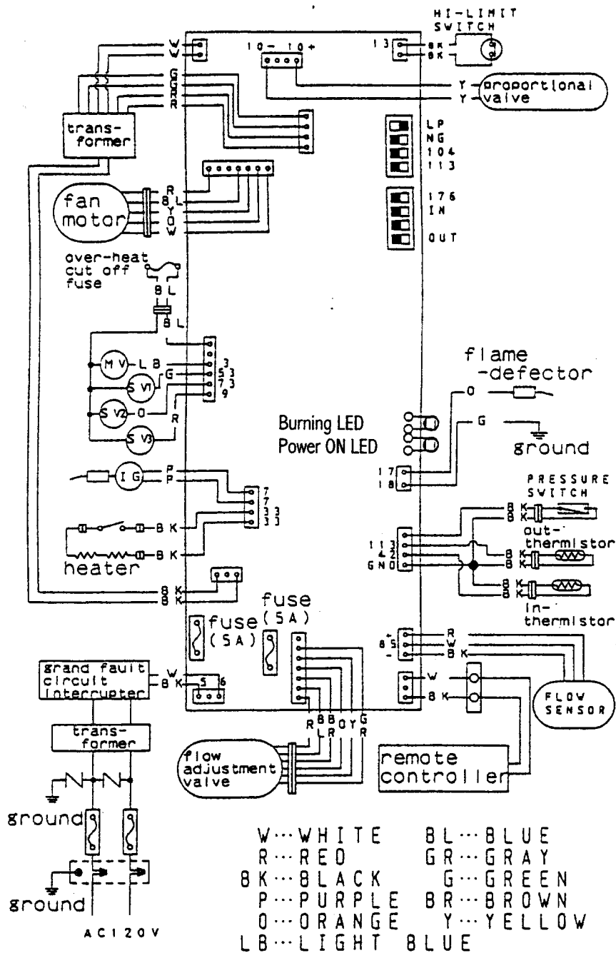
wiring Diagram
